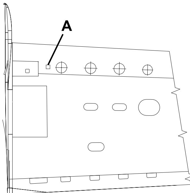
VIEW B-B
