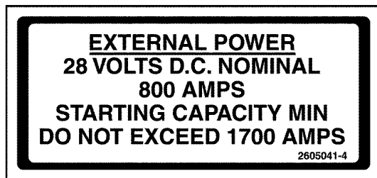
79 DETAIL B
