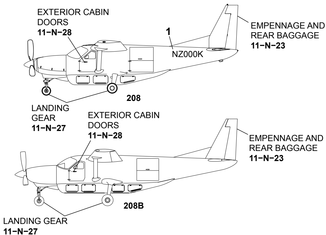
EXTERIOR SECTION ICAO NATIONALITY MARKS/COUNTRY DESIGNATIONS PLACARD LOCATIONS Figure 01. (Sheet 1)
