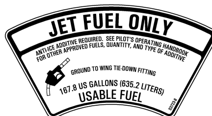
5 DETAIL B OUTBD FUEL FILL
